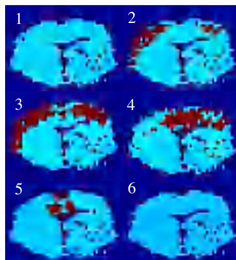
Fig.2. Position of tiers for the largest group shown in Fig. 1. The central pixel (top left) is in SI, and both SIs are primarily contained within the next two tiers, meaning that they are connected to the central pixel directly or via one intermediate pixel. Motor cortex is contained in tiers 4 and 5.
